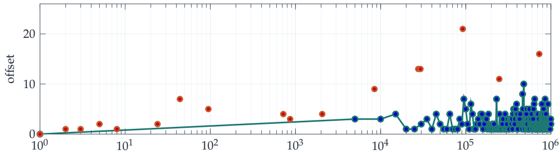
Each record gap strictly exceeds its incoming offset
