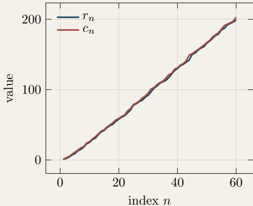
A. Exact interleaving of the axis terms
