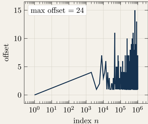
B. Offset \delta_n = c_n - r_n up to n = 10^6
