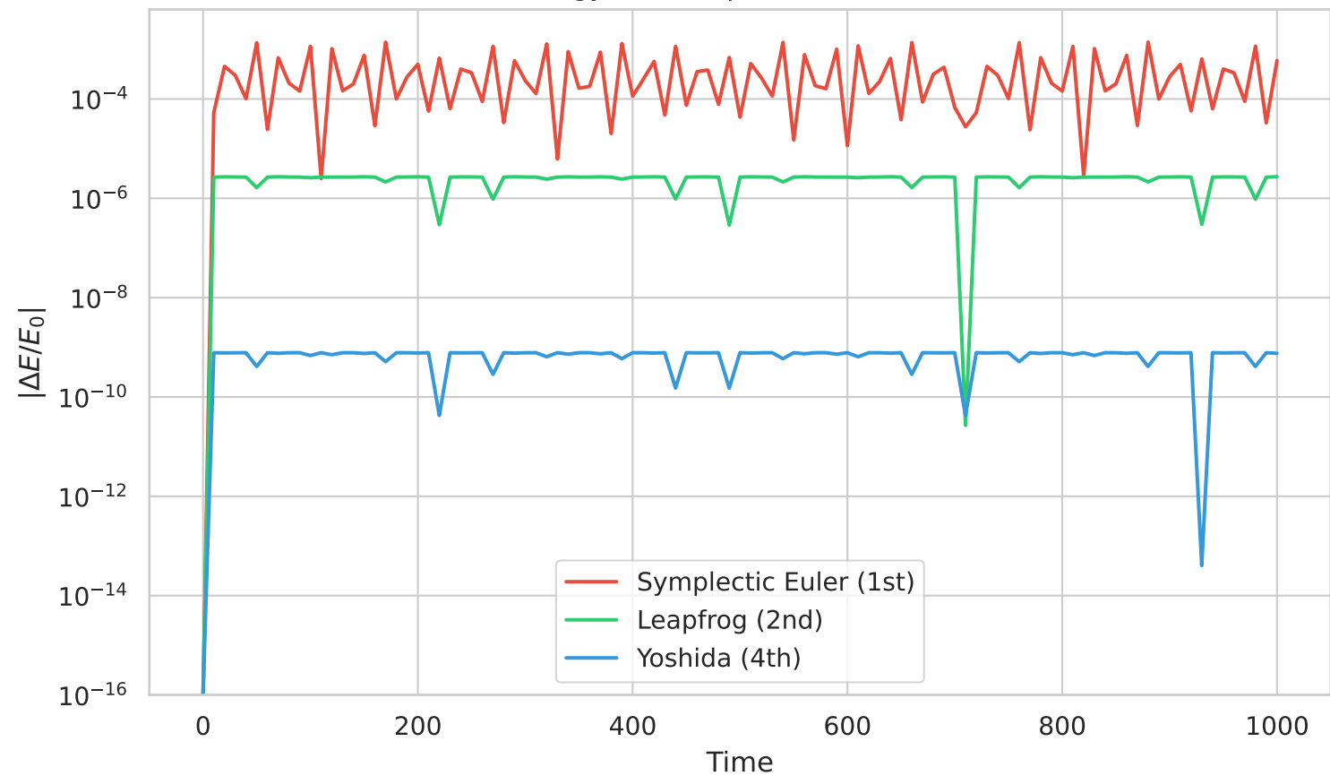
Energy Drift: Kepler Orbit (e=0.5)
