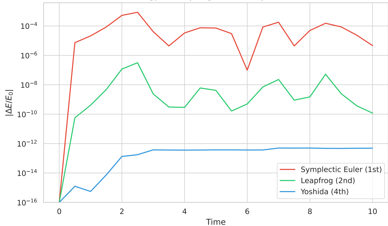
Energy Drift: Pythagorean 3-Body Problem
