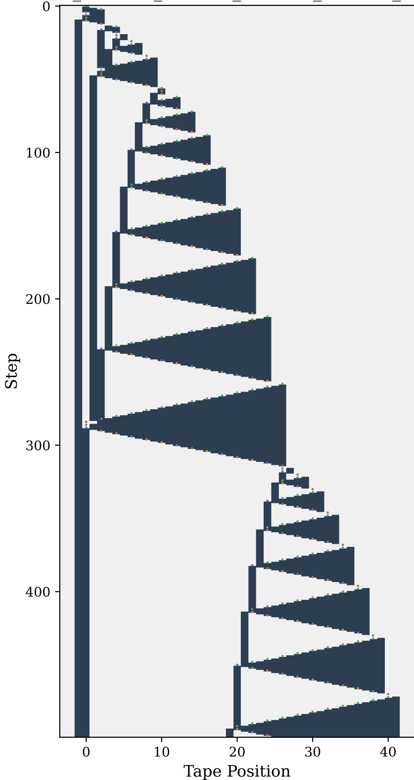
Space-Time Diagram (first 500 steps) 1RB0LD_1RC0RF_1LC1LA_0RE1RZ_1LF0RB_0RC0RE
