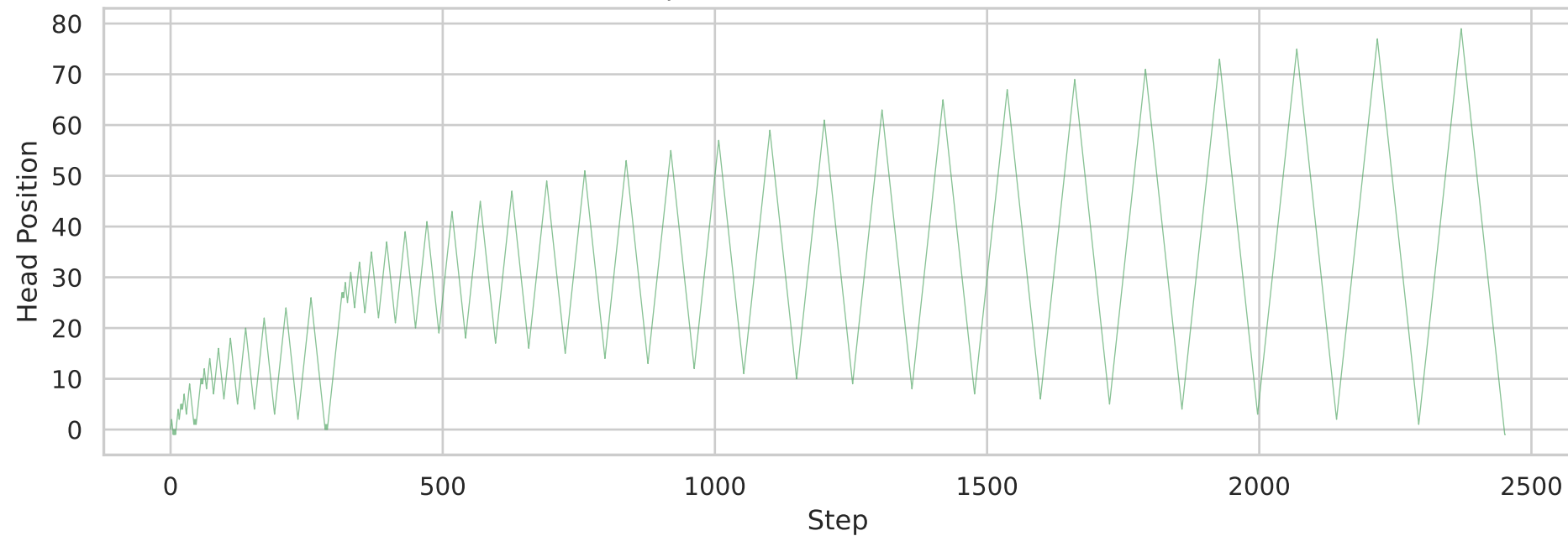
Tape Head Position Over Time
