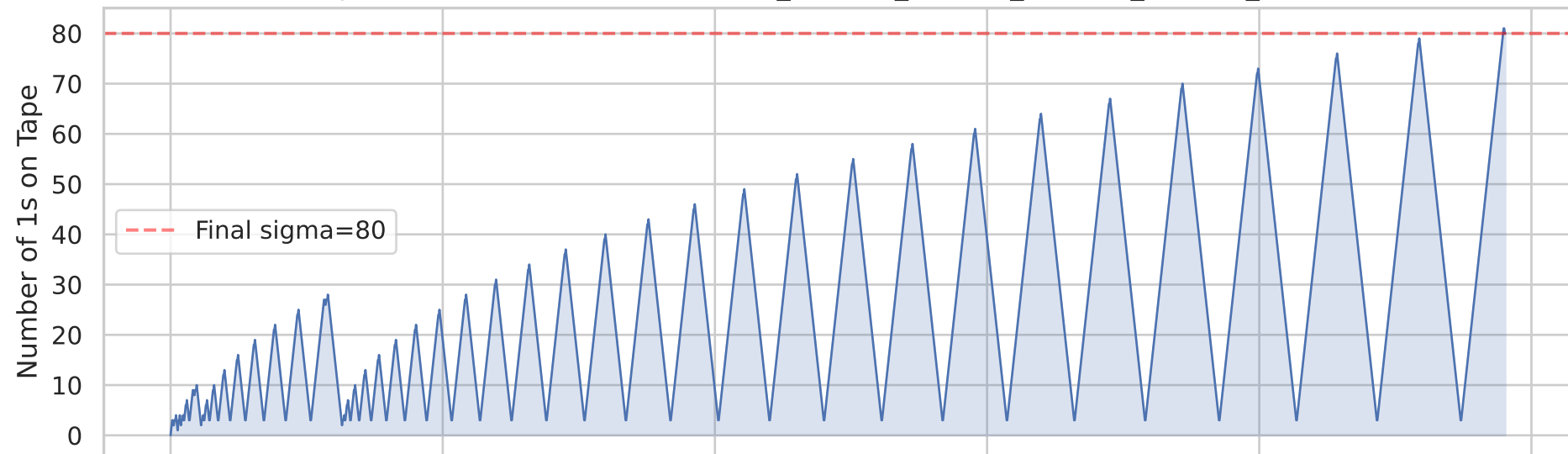
Tape Growth Over Time — 1RB0LD_1RC0RF_1LC1LA_0RE1RZ_1LF0RB_0RC0RE
