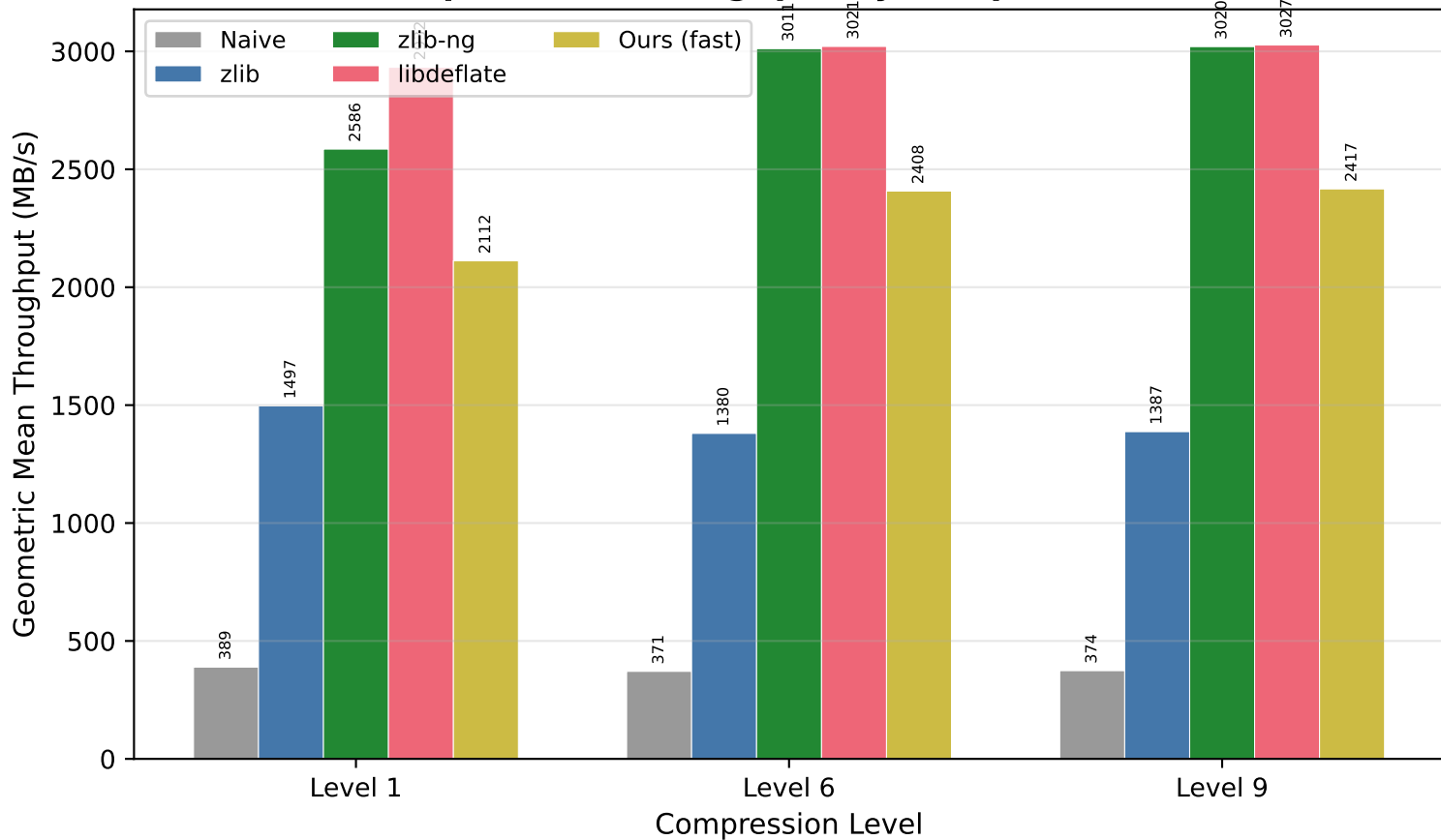
Decompression Throughput by Compression Level
