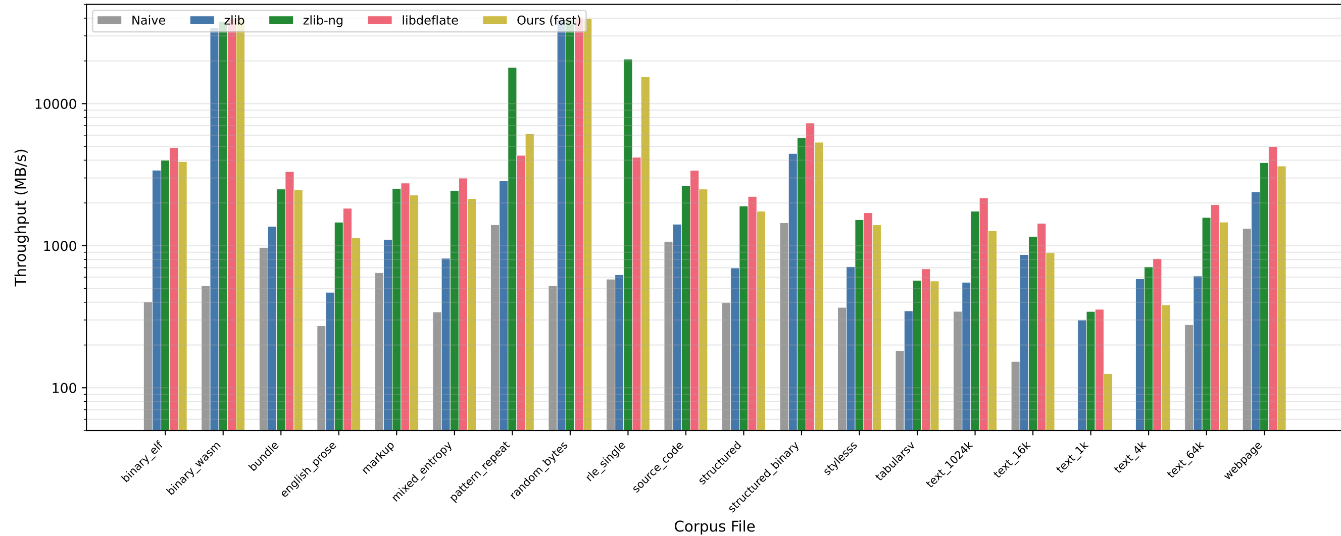
DEFLATE Decompression Throughput Comparison (Level 6)
