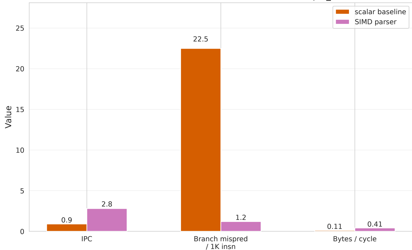
Hardware Performance Counters: Scalar vs SIMD (simple_uniform)
