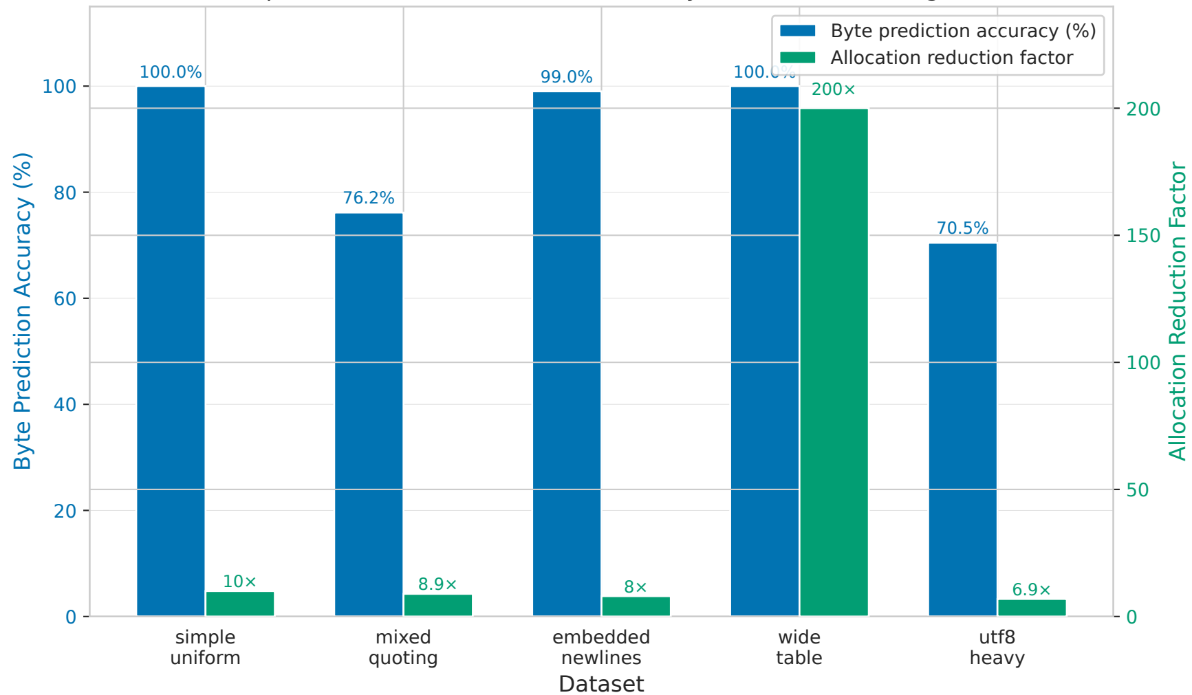
Speculative Field Detection: Accuracy & Allocation Savings
