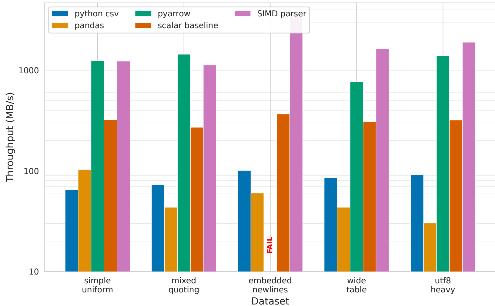
CSV Parser Throughput Comparison Across Datasets
