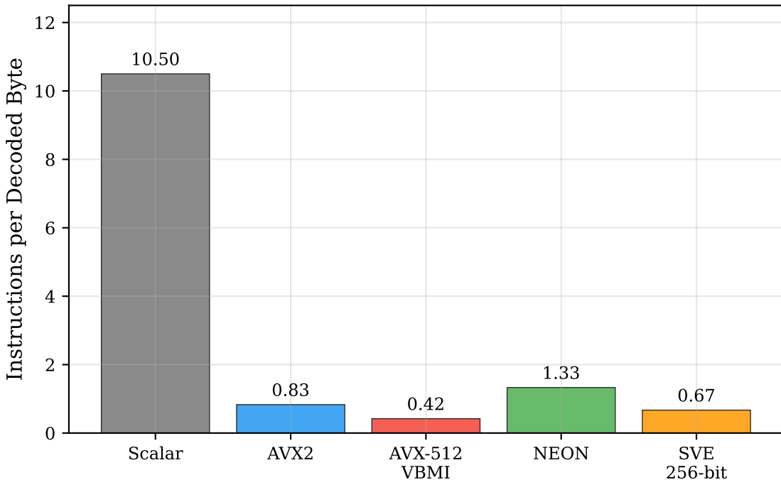
Instruction Efficiency by Implementation
