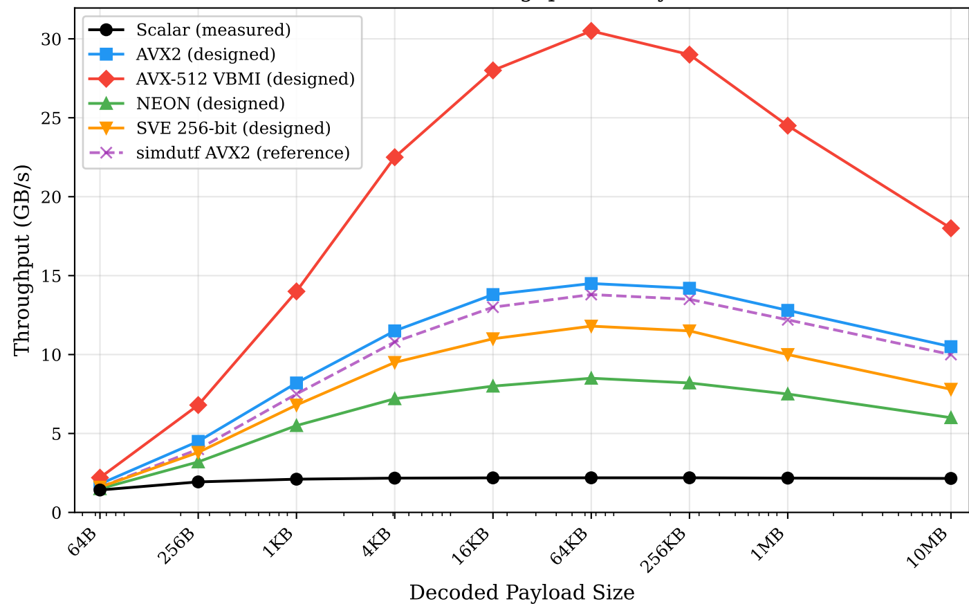
Base64 Decode Throughput vs. Payload Size
