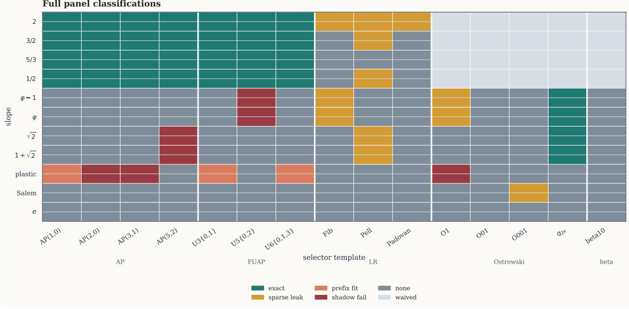
Figure 5: Full benchmark heatmap. Rows are the 11 tested slopes and columns are the 15 selector templates, for a total of 165 cells; 20 irrational-only cells are definition-driven waivers and the remaining 145 cells are executed cases. The exact-certified region is sharply localized: the entire AP/FUAP exact lane is rational, while the only sparse exact certificates occur on the even-convergent selector for \varphi - 1 , \varphi , \sqrt{2} , and 1 + \sqrt{2} . The figure is therefore a visual summary of the theorem/empirical split: periodic-gap selectors support a complete rational characterization, whereas sparse selectors exhibit a much narrower and explicitly non-classified survivor pattern.
