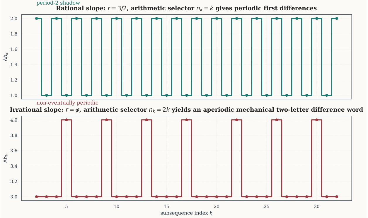
Figure 4: First-difference intuition behind Proposition 5.1. For a rational slope, the difference sequence along an arithmetic selector is eventually periodic; for an irrational slope such as \varphi it remains an aperiodic two-letter mechanical word. The proposition turns this picture into a proof: if the sampled values satisfied a recurrence, their bounded first differences would also satisfy a recurrence, hence would be eventually periodic by Lemma 3.4; Lemma 3.5 then forces the arithmetic-progression slope parameter to be rational.
