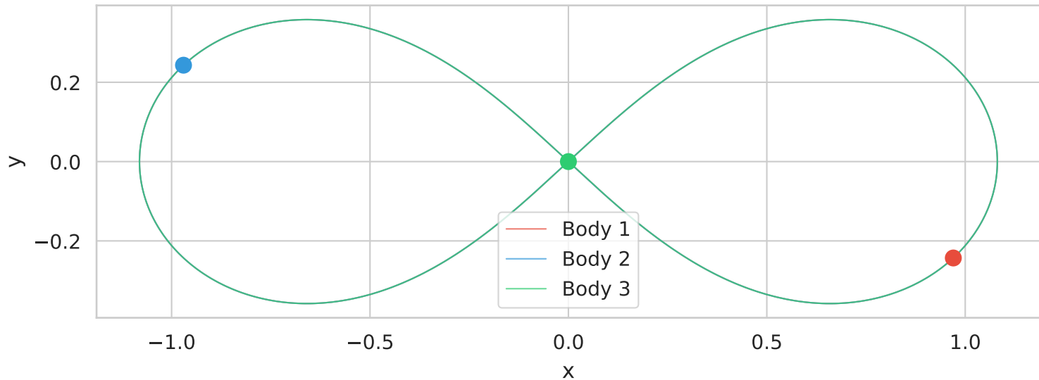
Figure-Eight Choreography (1 period, |\Delta E/E_0|=8.1\text{e-}15 )
