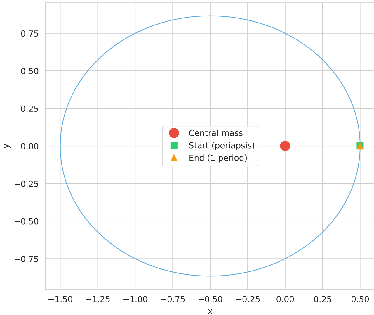
Kepler Orbit ( e=0.5 ), closure: 0.0511%
