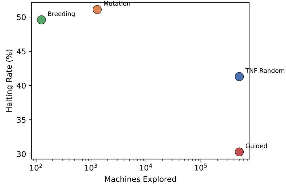
(b) Exploration vs. Halting Rate
