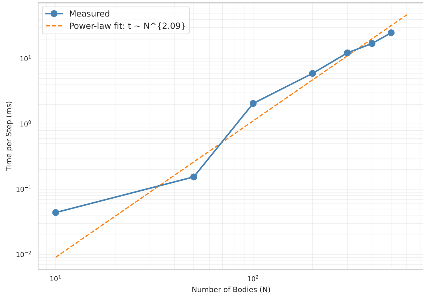
Baseline O(N^2) Scaling Verification (Fitted exponent: 2.09)
