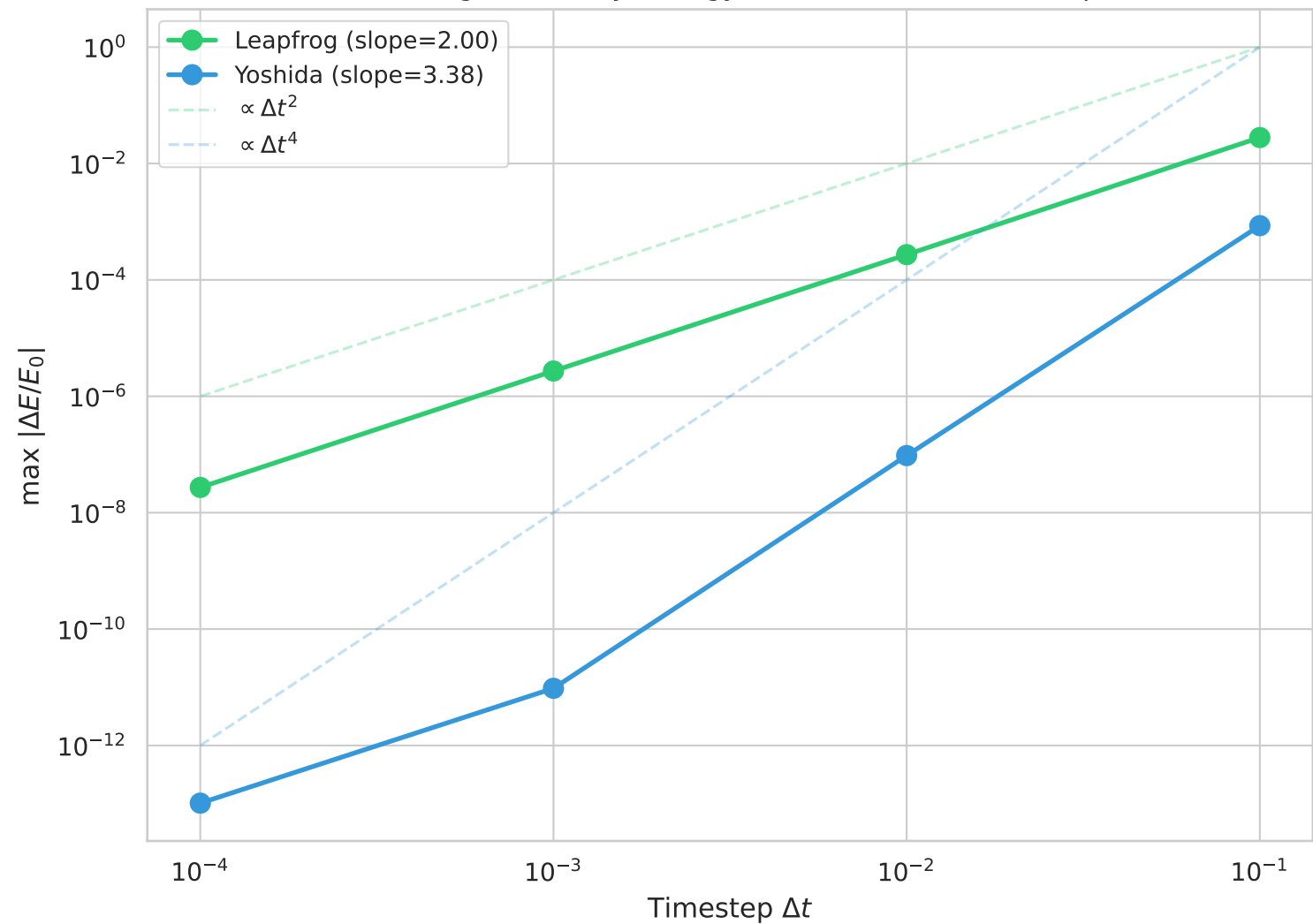
Convergence Study: Energy Conservation vs Timestep
