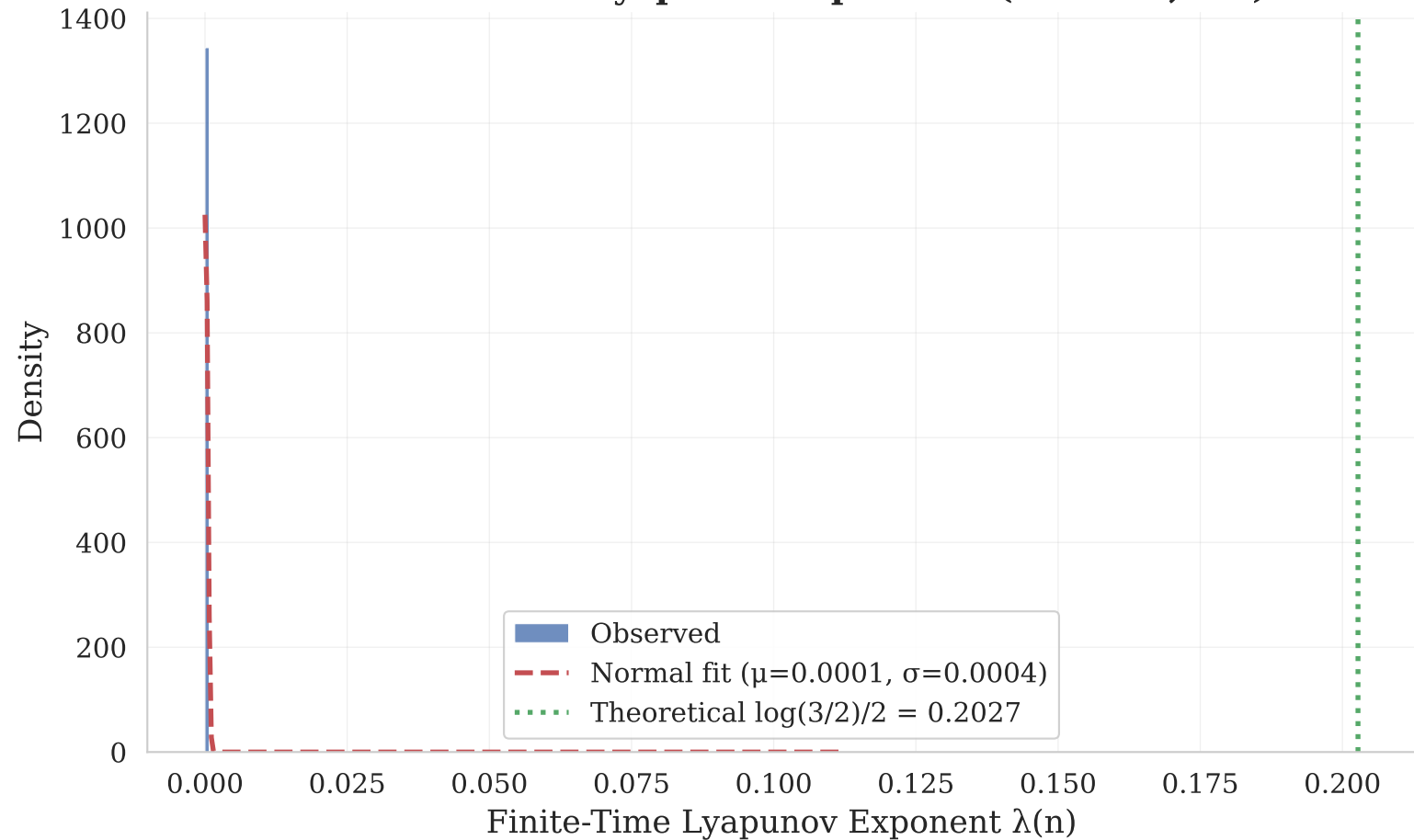
Distribution of Lyapunov Exponents (N = 100,000)
