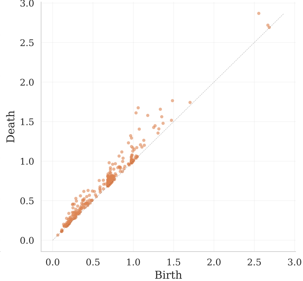
H1 Persistence Diagram
