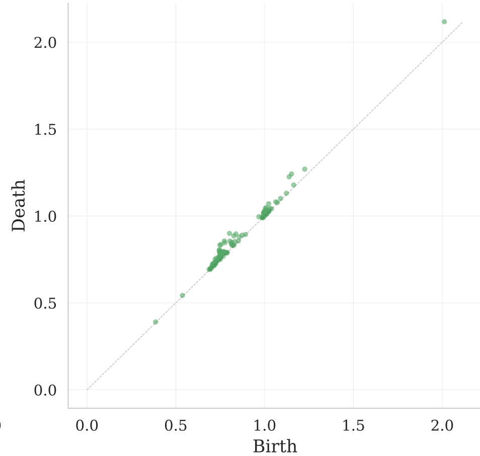
H2 Persistence Diagram
