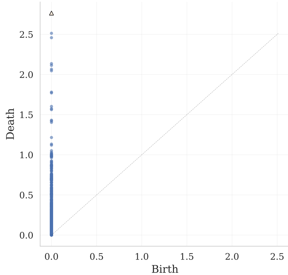
H0 Persistence Diagram
