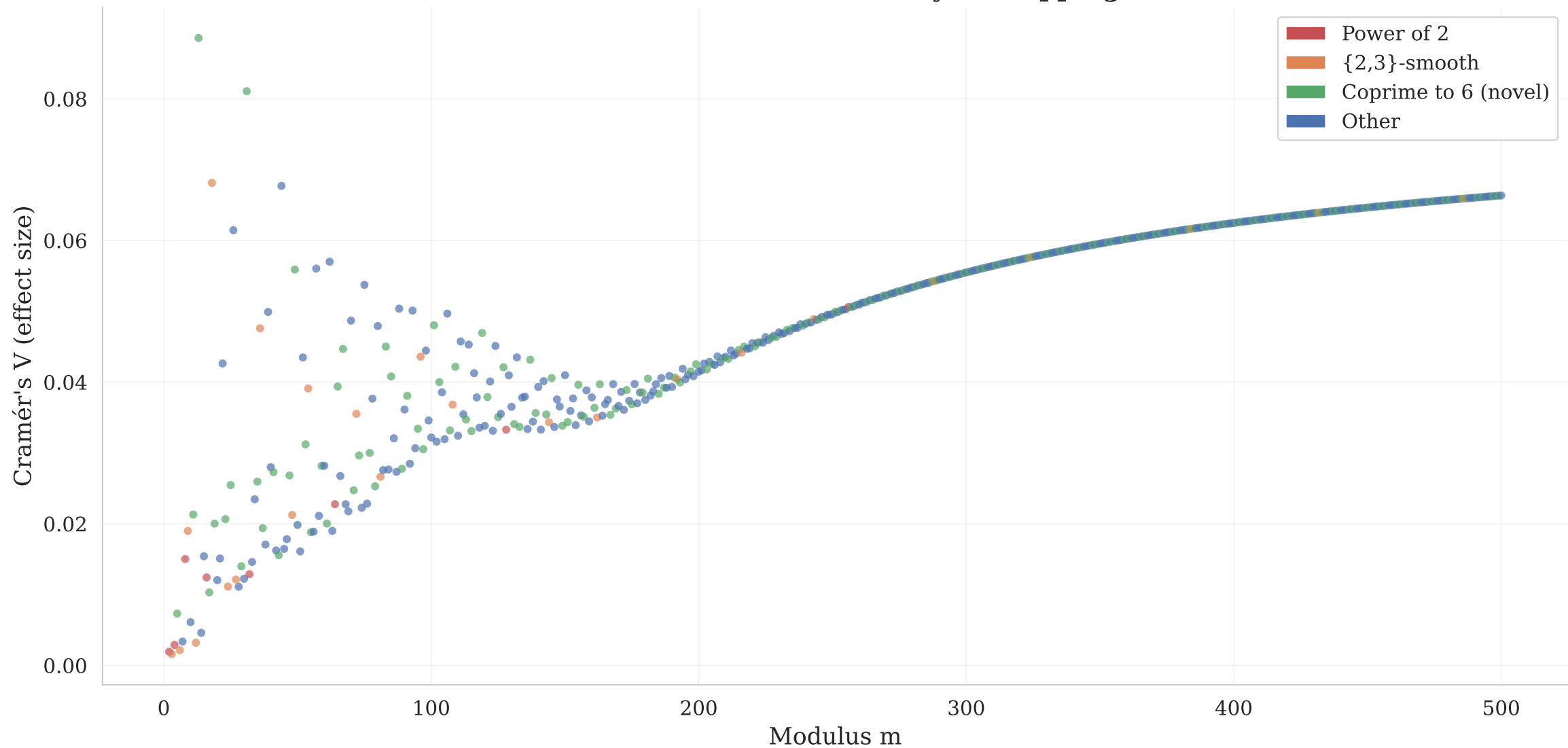
Modular Resonance Scan: Non-uniformity of Stopping Times mod m
