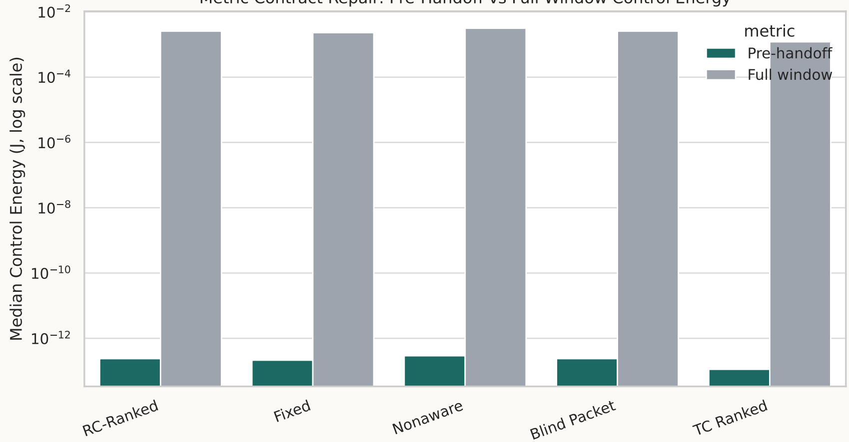
Metric Contract Repair: Pre-Handoff vs Full-Window Control Energy
