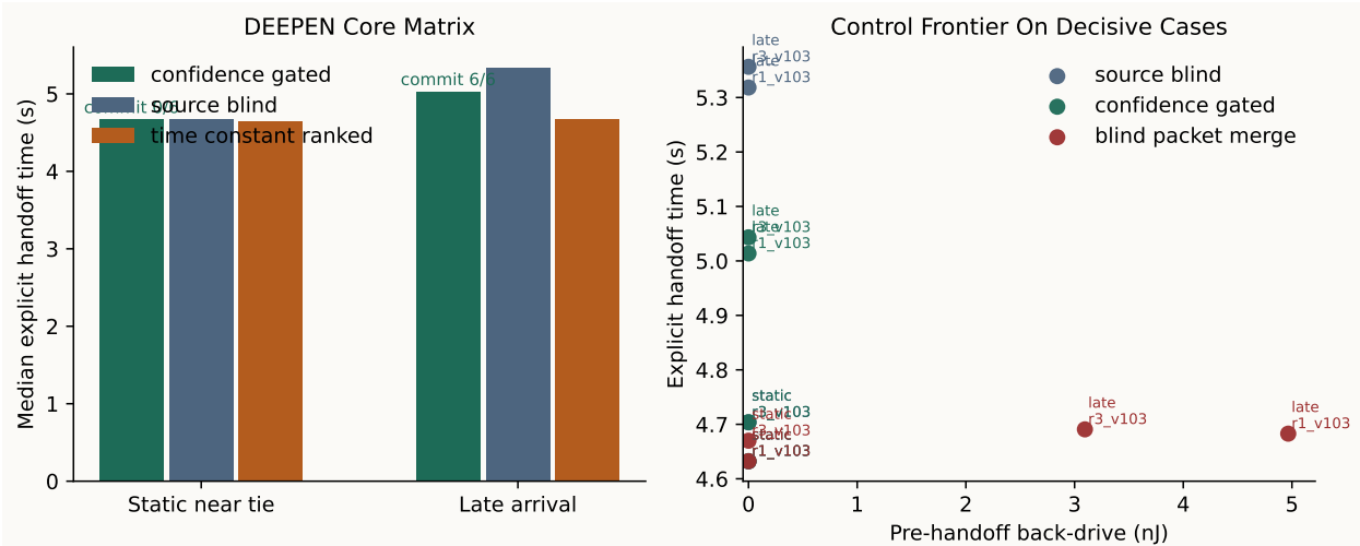
Figure 6: Central DEEPEN figure. Left panel: median explicit handoff times for the static and late near-tie families. The labels above the CONFIDENCE-GATED bars report commit counts. Static near ties produce 0/6 commits and essentially no gain over BLIND PACKET; late-arrival near ties produce 6/6 commits and a substantial median gain. Right panel: decisive same-scaffold control frontier on the four V_B - V_A = 3 mV cases. BLIND MERGE is fastest but incurs measurable wrong-way energy, BLIND PACKET is slowest but leak-free, and CONFIDENCE-GATED occupies the middle of the frontier while preserving zero measured backdrive. The figure is the paper’s core empirical result: the useful regime is temporal separability, not static ranking.
