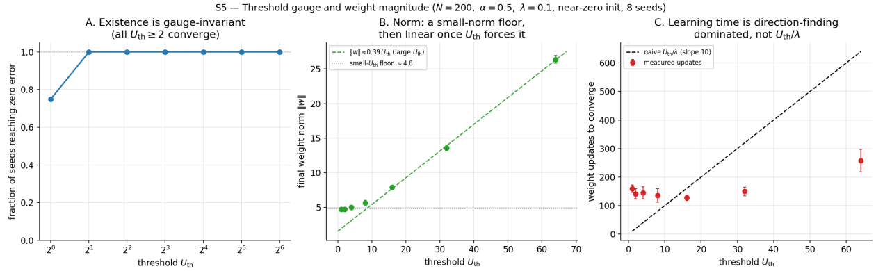
Figure 16: Threshold gauge and weight magnitude ( N = 200 , \alpha = 0.5 , \lambda = 0.1 , near-zero init, eight seeds). (A) Fraction of seeds reaching zero error vs U_{\text{th}} : existence is gauge-invariant ( U_{\text{th}} \geq 2 all converge). (B) Final \|w\| vs U_{\text{th}} : a small-norm floor ( \approx 4.8 ), then linear growth ( \approx 0.39 U_{\text{th}} ) once the threshold dominates. (C) Weight updates to converge vs U_{\text{th}} : flat (direction-finding dominated), far below the naive U_{\text{th}}/\lambda line.
