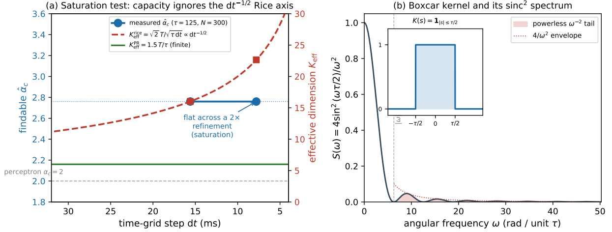
Measured (a): \hat{\alpha}_c = 2.76 at dt = 15.6 and 7.8 ms ( K_{\text{eff}}^{\text{rice}} moves 16.0 \rightarrow 22.7 , \times \sqrt{2} , yet \hat{\alpha}_c is unchanged).
