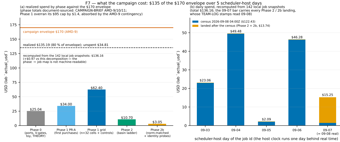
Figure 7: Realized spend by phase against the $170 envelope (left) and by scheduler-host day (right). The Phase 1 grid exceeded its cap by \approx \$1.4 after three zero-row timeouts and one bought control; Phase 2 and 2b came in under.
