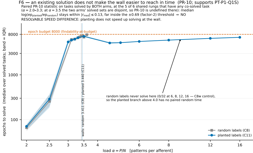
Figure 6: Median epochs to solve against \alpha for random and planted labels on the one-spike sinc cells (C8, C11), interquartile bands. At co-solved rungs the two arms take the same time to within 13%: planting does not speed up solving at the wall.
