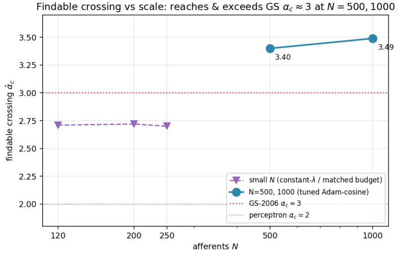
Figure 27: Findable crossing vs. scale. Small- N matched-budget values ( \approx 2.7 ) rise to \approx 3.4 ( N = 500 ) and 3.49 ( N = 1000 ) under the tuned learner, reaching and exceeding the GS benchmark \alpha_c \approx 3 at the faithful scales.
