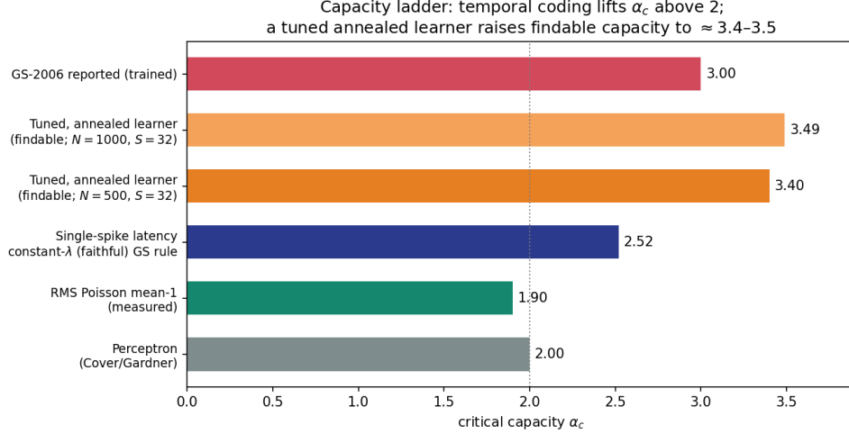
Figure 1: The capacity ladder framing this study: \alpha_c = 2 (perceptron) \rightarrow constant-step trained \approx 2.5 \rightarrow tuned annealed learner with a findable crossing \approx 3.4 –3.5 at the faithful scales. On the single-spike latency ensemble the bare Gütig–Sompolinsky-inspired rule reaches only a findable \alpha_c \approx 2.5 at N = 500 ; Sections 9–15 establish each rung and show a tuned, annealed learner reproducibly reaches and exceeds the GS load, with a findable half-crossing \approx 3.4 at N = 500 and 3.49 at N = 1000 ( S = 32 ; §15). This is a findability result; the existence capacity (a trainer-independent Gardner oracle) is left open.
