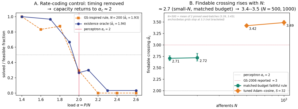
Figure 25: Controls (regenerated from committed artifacts: results/t2b_synchrony/ and analysis/data/audit_stats.json ). (A) Rate-coding limit (timing removed): both the trainer-independent existence oracle ( \hat{\alpha}_c = 1.94 ) and the GS-inspired rule ( N=200 , drive-peak read-out, \hat{\alpha}_c = 1.93 ) cross \frac{1}{2} near the perceptron value \alpha_c = 2 — the single-spike lift is a property of the code, not the pipeline. (B) The findable crossing rises with N : matched-budget \hat{\alpha}_c \approx 2.7 at small N ( t2a_faithful : 2.71, 2.72 at N=120, 200 ) to \approx 3.4 ( N=500 ; mean of the two pinned seed-batches) and 3.49 ( N=1000 ) under the tuned S=32 campaign (§15). Error bars are isotonic-bootstrap 95% CIs.
