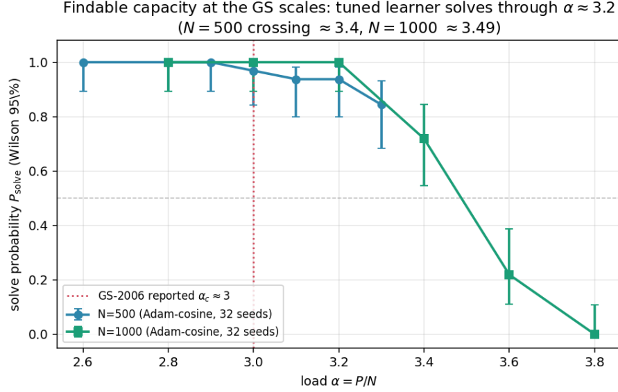
Figure 26: Findable capacity at the GS scales. P_{\text{solve}}(\alpha) for the tuned Adam-cosine learner at N = 500 and N = 1000 ( S = 32 , Wilson 95%). Both solve reliably through \alpha \approx 3.2 ; the half-crossings ( \approx 3.4 at N = 500 , 3.49 at N = 1000 ) sit above the GS-reported \alpha_c \approx 3 (red).
