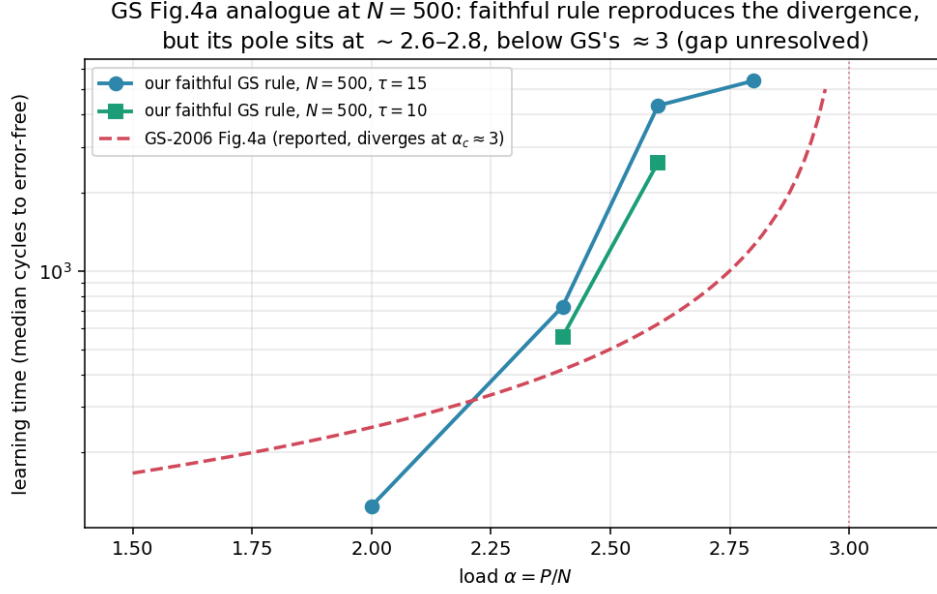
Figure 28: Head-to-head with the original benchmark (GS-2006 Fig. 4a). Median learning time (cycles to error-free classification) vs. load for our faithful GS rule at N = 500 ( \tau = 15 and \tau = 10 ), with the GS-2006 reported divergence ( \propto 1/(\alpha_c - \alpha) , \alpha_c \approx 3 ) overlaid (red dashed). The faithful rule reproduces the divergence shape , but its pole lies at \alpha \approx 2.6\text{--}2.8 and its cycle counts run \sim 3\times higher than GS's, so the exact \alpha_c \approx 3 of the original rule is not yet reproduced — the central open item.
