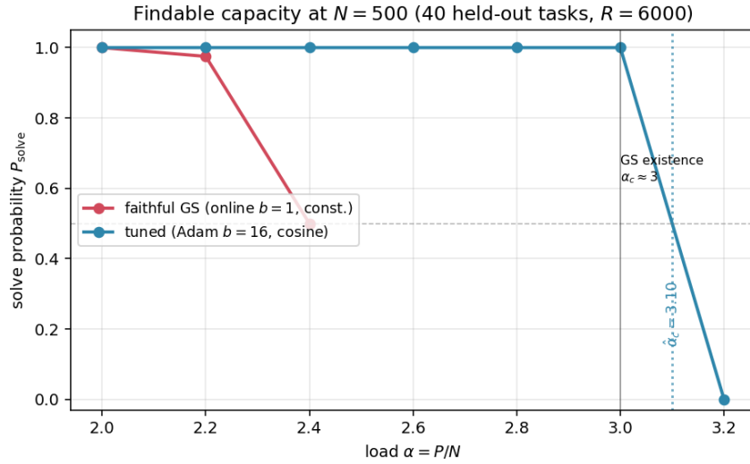
Figure 22: Findable capacity at N = 500 on 40 held-out tasks. The faithful Güting–Sompolsky rule crosses P_{\text{solve}} = \frac{1}{2} near \alpha \approx 2.4 ; the tuned learner (Adam, b=16 , cosine) solves every task through \alpha = 3.0 and crosses at \hat{\alpha}_c = 3.10 — the existence value \alpha_c \approx 3 (vertical line). The findability gap is essentially eliminated.
