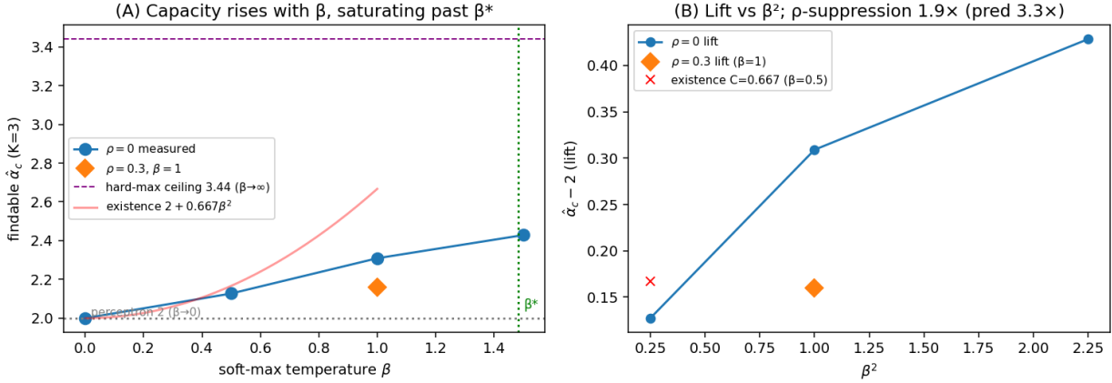
Model #5 — soft-max( \beta ) capacity: convex \rightarrow shattered knob ( K=3 , N=250 )
