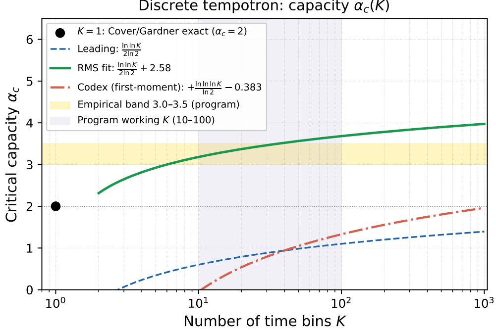
Figure 1: Capacity \alpha_c(K) for the discrete binned tempotron. Dot: the exact K = 1 anchor ( \alpha_c = 2 ) from Cover’s theorem. Dashed blue: leading term (\ln \ln K)/(2 \ln 2) only (RMS EVT). Solid green: RMS small- K fit (\ln \ln K)/(2 \ln 2) + 2.58 (the additive constant 2.58 is a fit, not a derived asymptotic, per Section 5.1). Dash-dotted red: first-moment/cluster next term (\ln \ln K)/(2 \ln 2) + (\ln \ln \ln K)/\ln 2 - 0.383 from the codex cross-check (Section 5.1); valid for K \gtrsim 4 . Gold band: empirical range 3.0–3.5 measured in the program (single-learner scaling). Purple band: program’s working K range (10–100).
