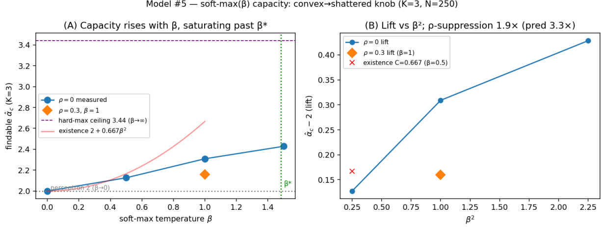
Figure 2: (A) \hat{\alpha}_c rises from the perceptron value 2 with \beta , saturating past \beta^* toward the hard-max ceiling. (B) lift vs. \beta^2 and the \rho -suppression.
