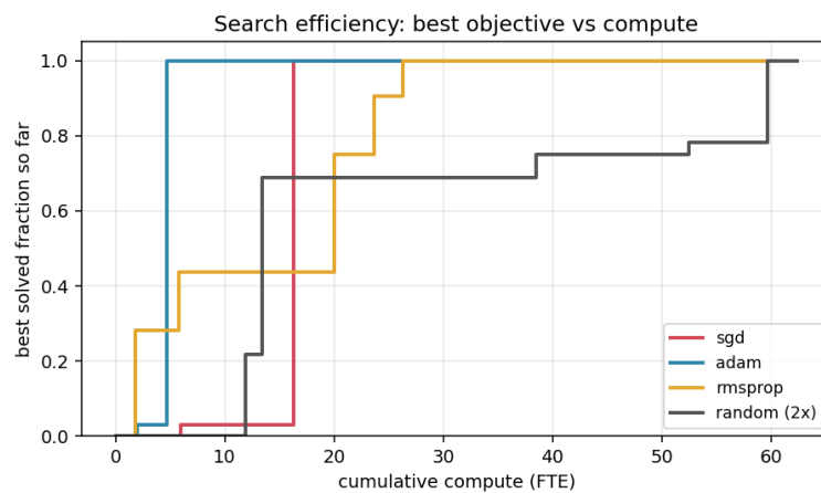
Figure 21: Search efficiency: best solved fraction attained versus cumulative compute (FTE) per arm (random baseline at 2\times budget). Guided search reaches the optimum with less compute than random.
