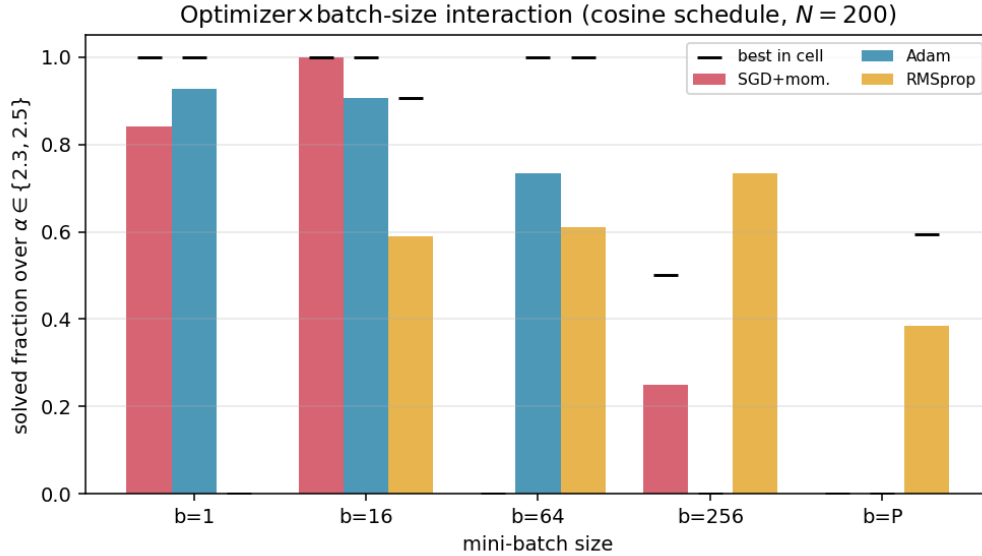
Figure 20: Optimiser \times batch-size interaction (cosine schedule). Bars are the mean solved fraction over completed trials in each cell; black ticks the best in the cell. SGD+momentum (small/online) and RMSprop (large batch) prefer opposite regimes; Adam spans the middle; nobody tolerates full-batch.
