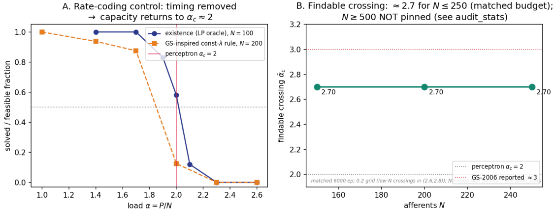
Figure 25: Controls. Both panels are currently figure-asserted from uncommitted lab-job summaries (provenance gap, §17, Tier-2); the committed v12-j3*_synchrony folders are failed runs. (A) Rate-coding limit (timing removed): both the trainer-independent existence oracle ( N=100 ) and the GS-inspired constant- \lambda rule ( N=200 , drive-peak read-out) cross \frac{1}{2} near the perceptron value \alpha_c = 2 — the single-spike lift is a property of the code, not the pipeline. (B) The single-spike findable crossing grows with N over the small- N range: matched 6000-epoch \hat{\alpha}_c \approx 2.7 for N \leq 250 . (Grid spacing 0.2, so low- N crossings localise to (2.6, 2.8); an earlier 4000-epoch run read \approx 2.4 at N = 150 — the crossing is budget- as well as N -dependent. N \geq 500 is not pinned and is omitted.)
