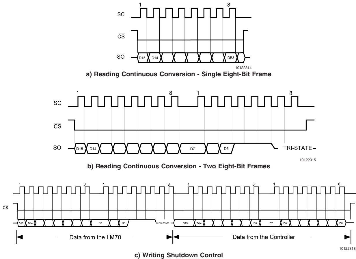
FIGURE 7. Timing Diagrams
