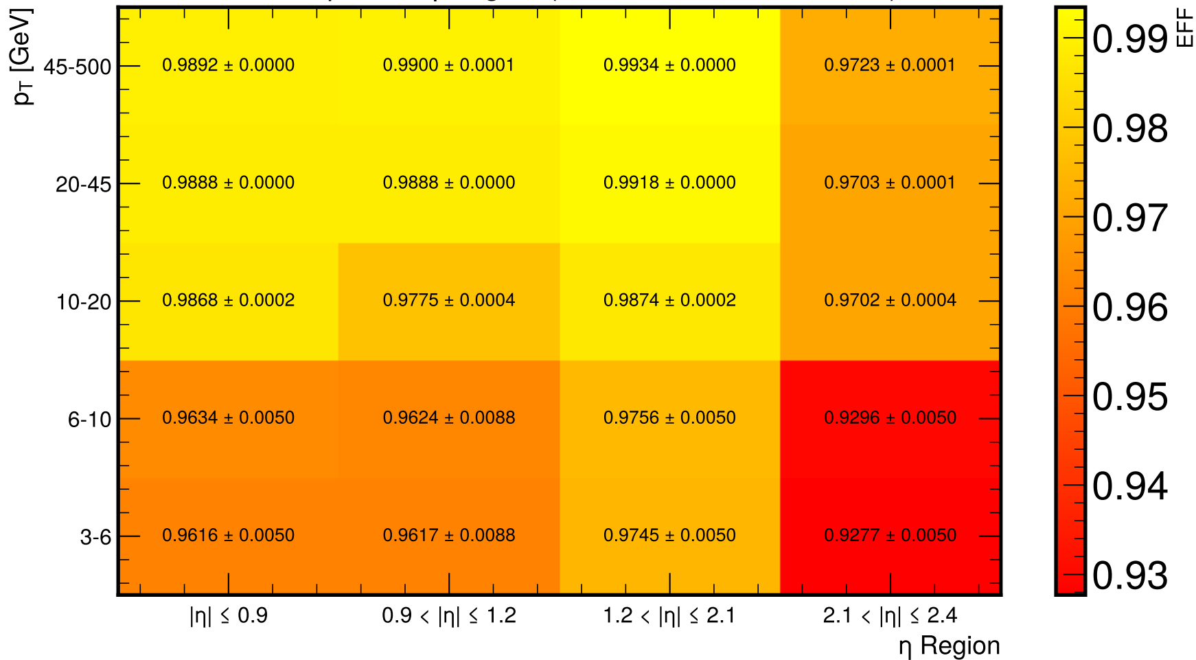
EFF vs. p_T and \eta Region (DATA Muon GoldID 2018)
