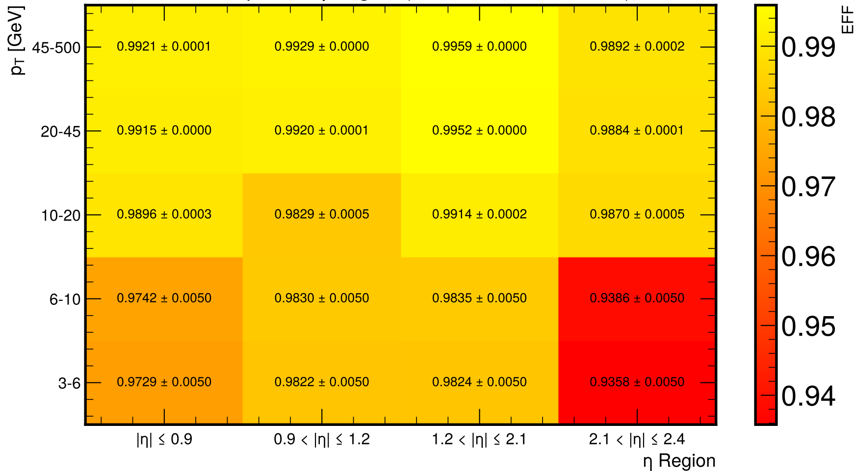
EFF vs. p_T and \eta Region (MC Muon GoldID 2018)
