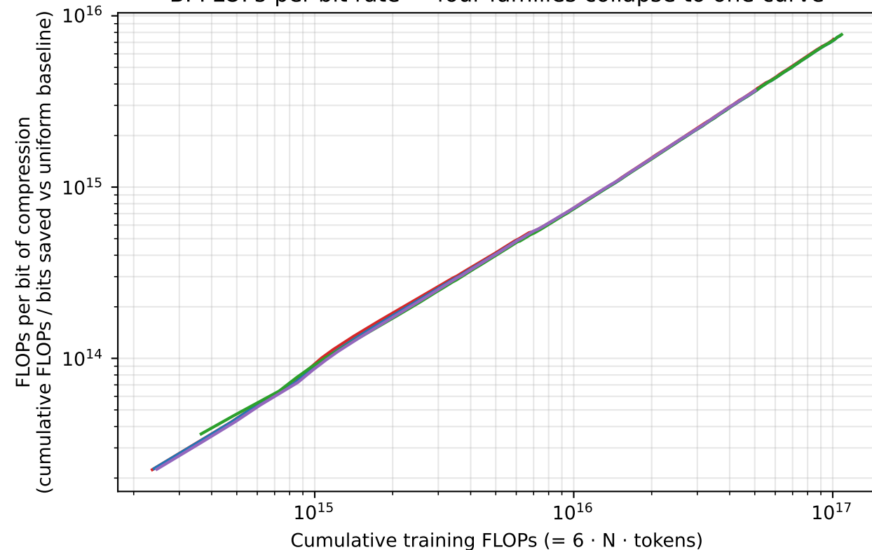
B. FLOPs-per-bit rate — four families collapse to one curve
