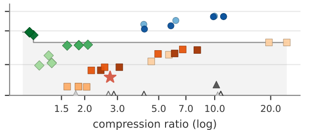
Synthetic columns
