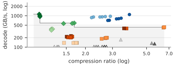
Real-world columns
