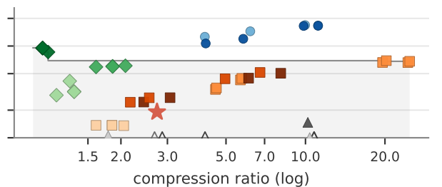
Synthetic columns
