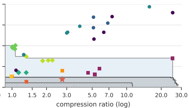
Generated columns
