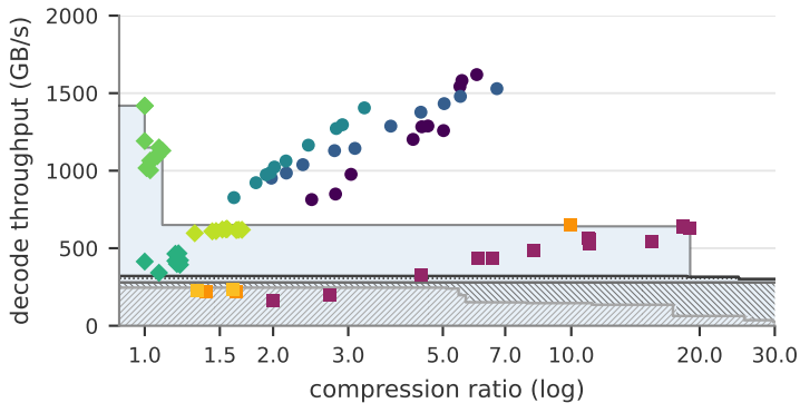
Real-world columns
