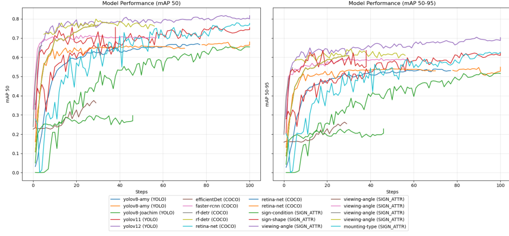
Figure 12: Comparison of mAP across different detectors
