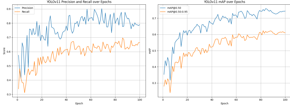
Figure 9: YOLOv11 Training Metrics.
