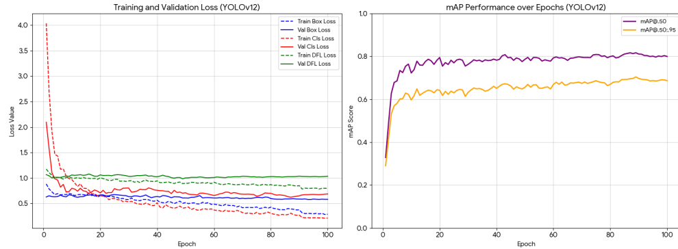
Figure 10: YOLOv12 Training Metrics.
