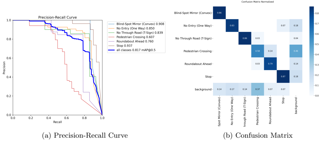
Figure 11: Precision-Recall Curve and Confusion Matrix for YOLOv12
