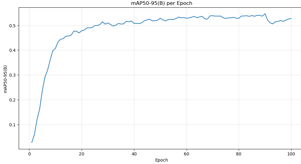
Figure 8: YOLOv8 mAP@0.50:0.95 per Epoch
