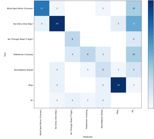
Figure 5: RF-DETR Confusion Matrix
