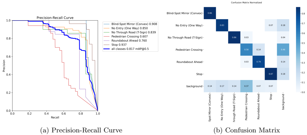
Figure 6: Precision-Recall Curve and Confusion Matrix for YOLOv12
