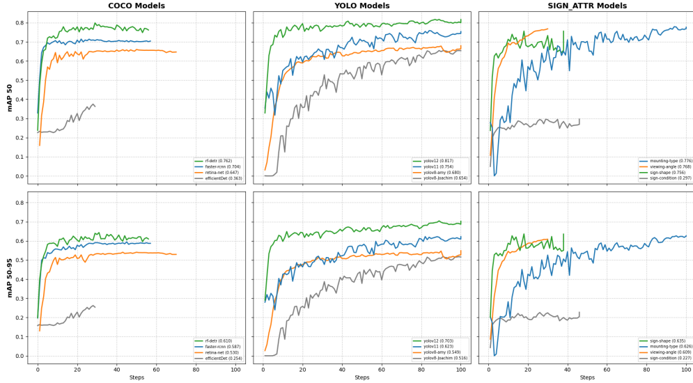
Figure 12: Comparison of mAP across the different models, grouped by category
