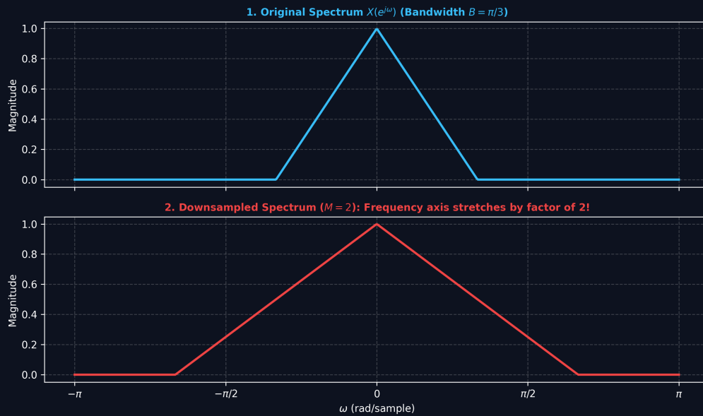
Figure 1: Downsampling (Decimation) Frequency Spectrum: Frequency Axis Expansion and Anti-Aliasing Requirement.
