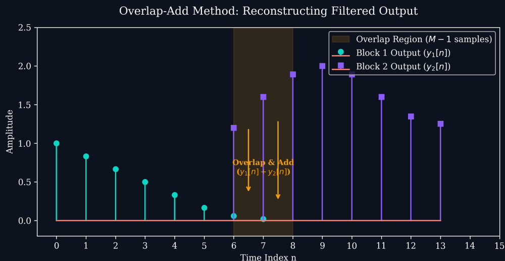
Figure 5: Overlap-Add block processing.
