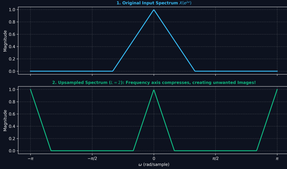
Figure 2: Upsampling (Interpolation) Spectrum: Zero-Insertion Spectral Compression and Anti-Imaging Filter.
