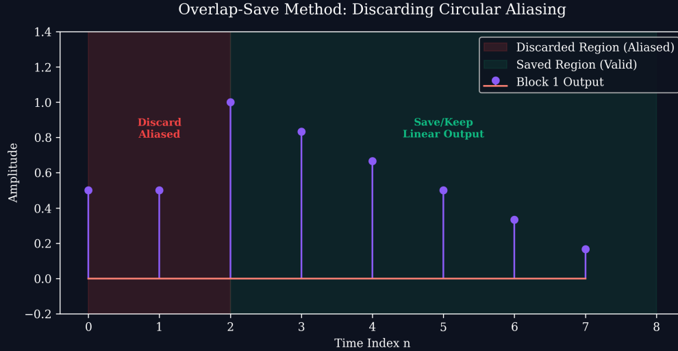
Figure 6: Overlap-Save block processing.
