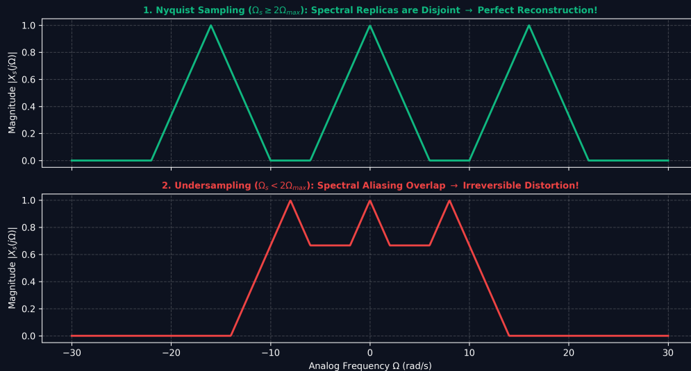
Figure 4: Sampling Replication and Spectral Aliasing using Triangles.
