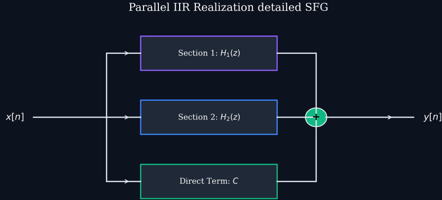
Figure 1: Iir Parallel Sfg
