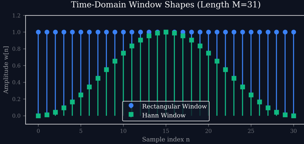
Figure 1: Window Shapes
