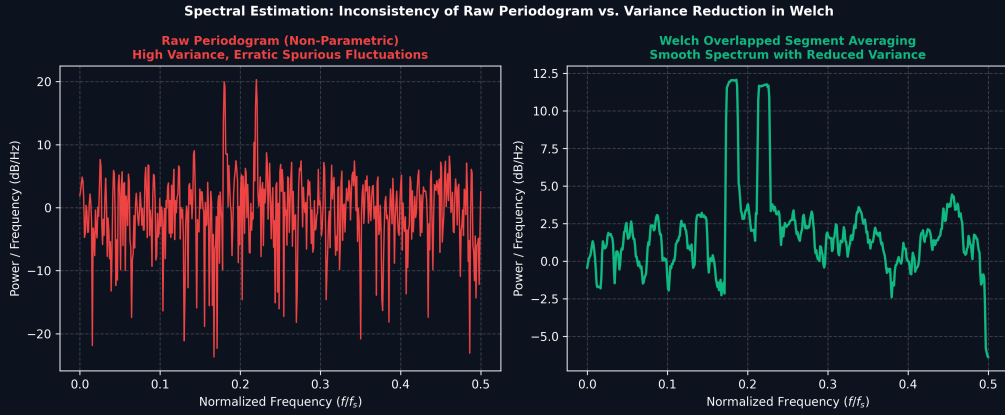
Figure 1: Spectral Estimation: Inconsistent Raw Periodogram Variance vs. Smooth Welch Segment Averaging.
