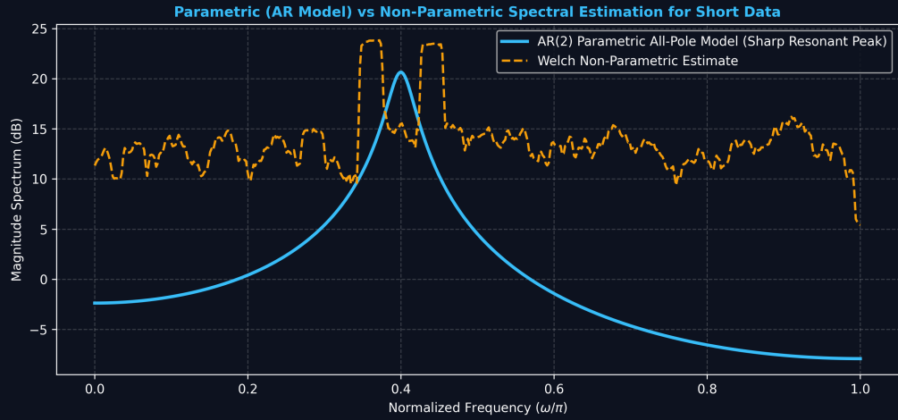
Figure 2: Parametric Autoregressive (AR) All-Pole Model vs. Non-Parametric Welch Spectral Resolution.
