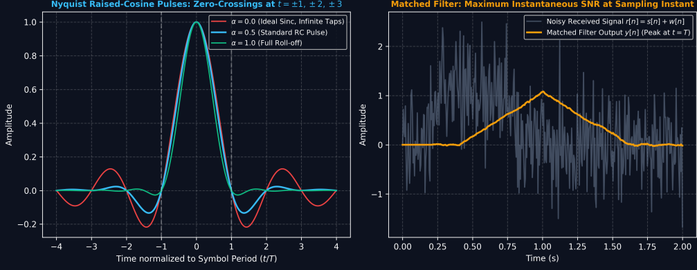
Figure 1: Nyquist Raised-Cosine Zero-ISI Pulses and Matched Filter Output Peak Instantaneous SNR.
