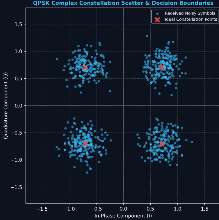
Figure 2: QPSK Complex Constellation Scatter Diagram with Noise and Decision Boundaries.
